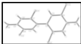
Fig. 1. Molecular structure showing 50% probability displacement ellipsoid.
